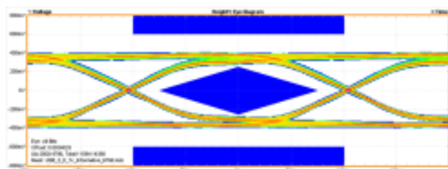
Figure 13. Output Eye Diagram Without the TPD4EUSB30 (5 Gbps Data Rate)
