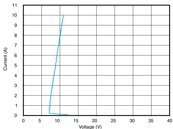
Figure 4. D+, D- Transmission Line Pulser Plot for TPD2EUSB30 (100 ns Pulse, 10 ns Rise Time)
