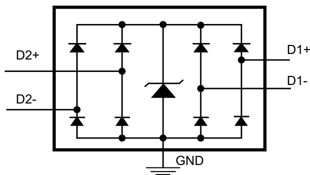
TPD2EUSB30/A Circuit
