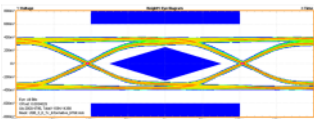
Figure 14. Output Eye Diagram with the TPD4EUSB30 (5 Gbps Data Rate)
