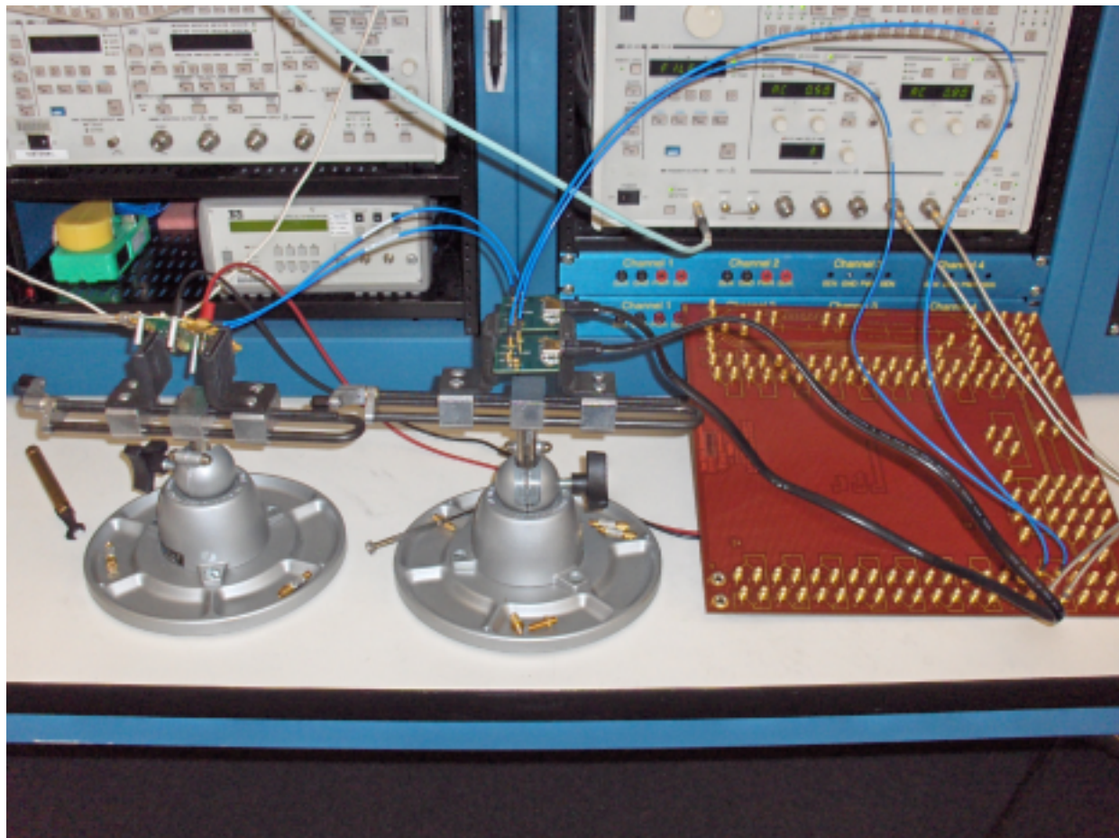
Figure 10. Lab Setup for the Eye-Pattern Measurement with TPDxEUSB30/A
