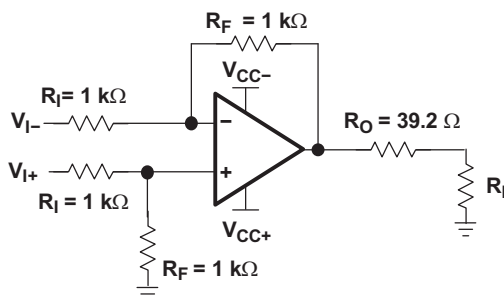
Figure 17. Differential Input With A Noninverting Gain Of 2V/V
