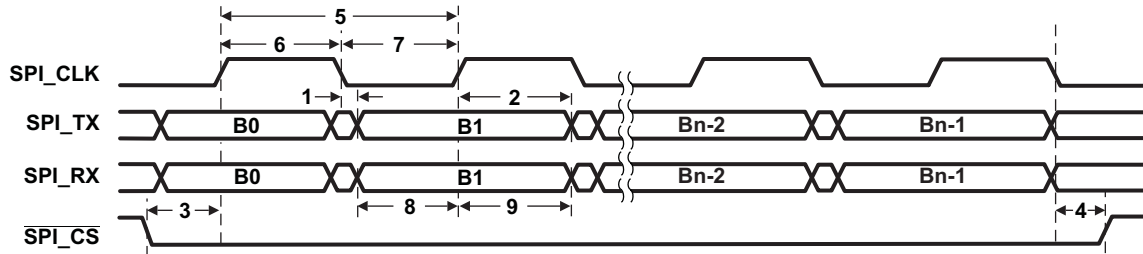
Figure 6-26. SPI Mode 0 Transfer (CKP n = 0, CKPH n = 0)
