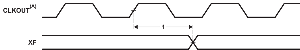
Figure 6-13. XF Timings
