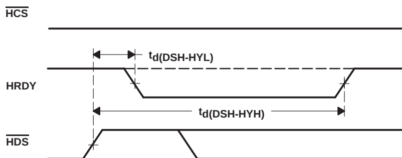
Figure 32. \text{HRDY} Signal When \overline{\text{HCS}} is Always Low
