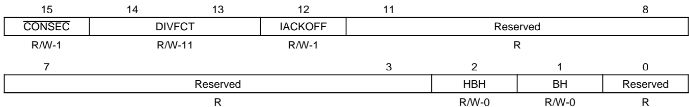
Figure 3-7. Bank-Switching Control Register (BSCR) [MMR Address 0029h]
