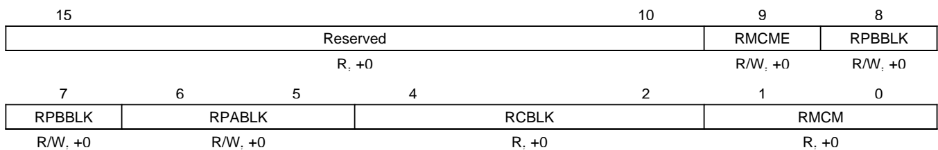
Figure 3-12. Multichannel Control Register 1x (MCR1x)
