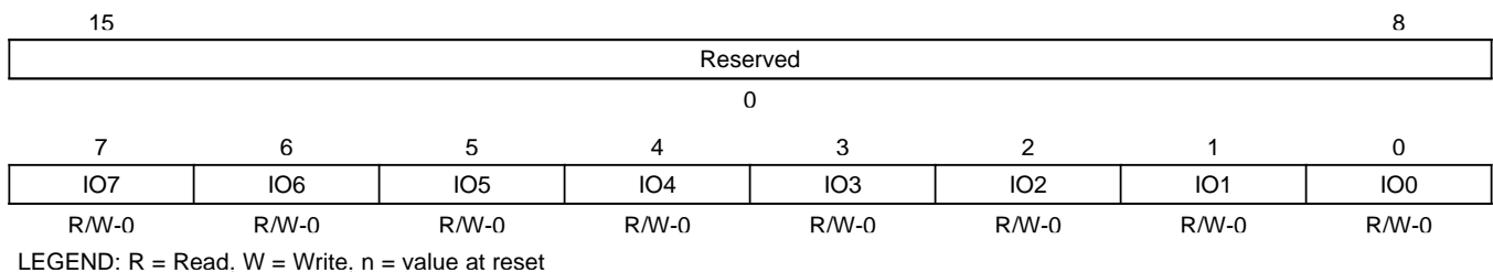
Figure 3-24. General-Purpose I/O Status Register (GPIOSR) [MMR Address 003Dh]
