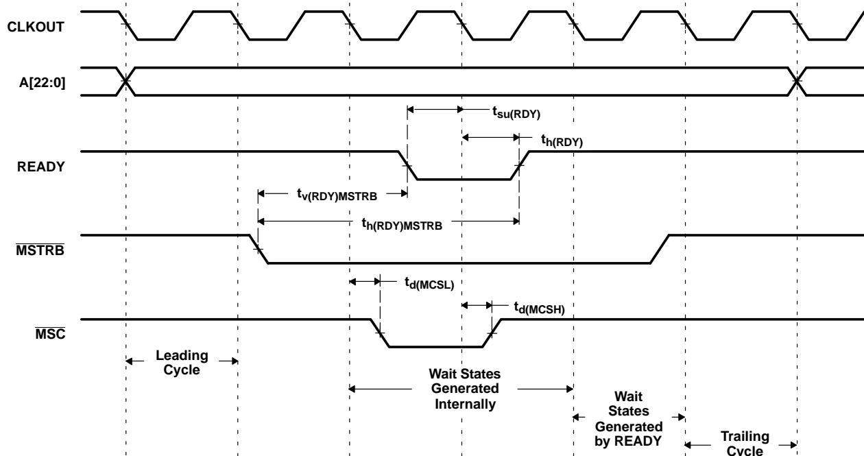
Figure 5-10. Memory Read With Externally Generated Wait States
