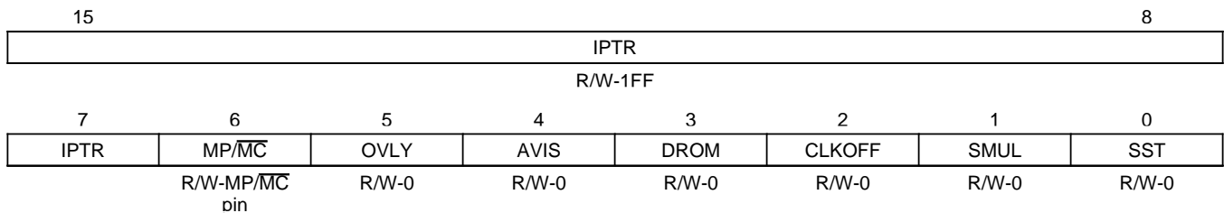
Figure 3-4. Processor Mode Status Register (PMST)
