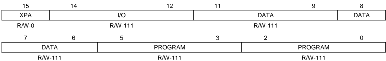
Figure 3-5. Software Wait-State Register (SWWSR) [Memory-Mapped Register (MMR) Address 0028h]
