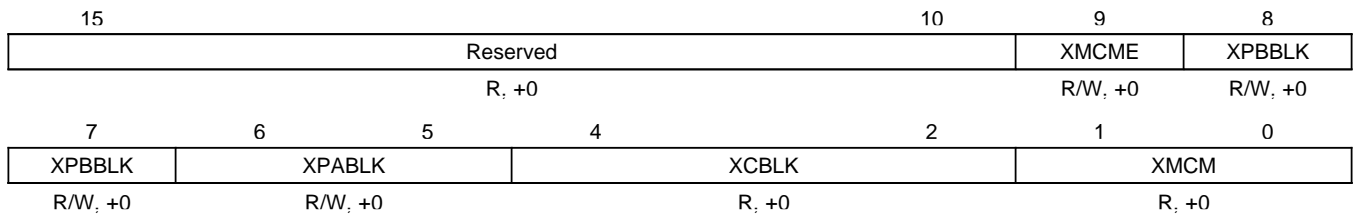
Figure 3-11. Multichannel Control Register 2x (MCR2x)
