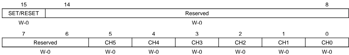
Figure 3-19. DMA Channel Enable Control Register (DMCECTL)
