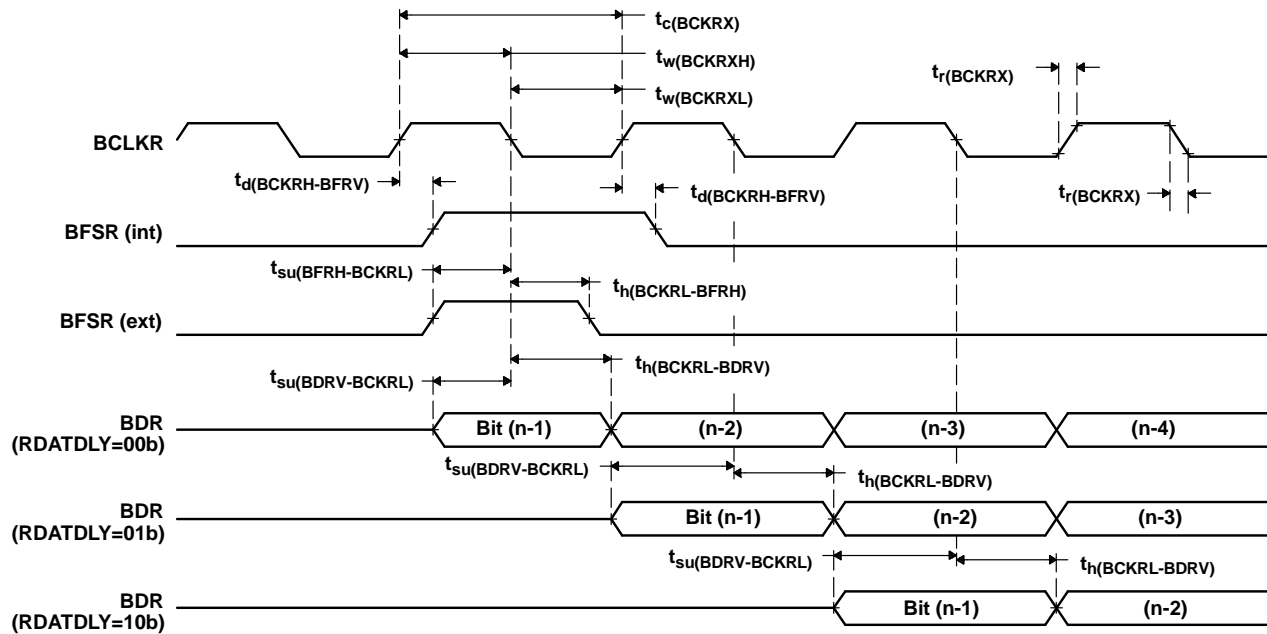
Figure 5-21. McBSP Receive Timings
