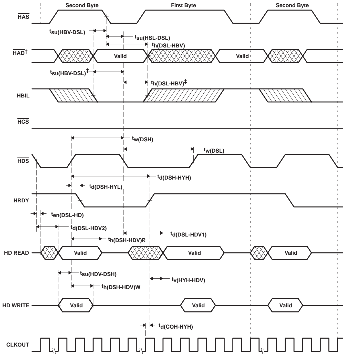
Figure 35. Using \overline{HDS} to Control Accesses ( \overline{HCS} Always Low)
