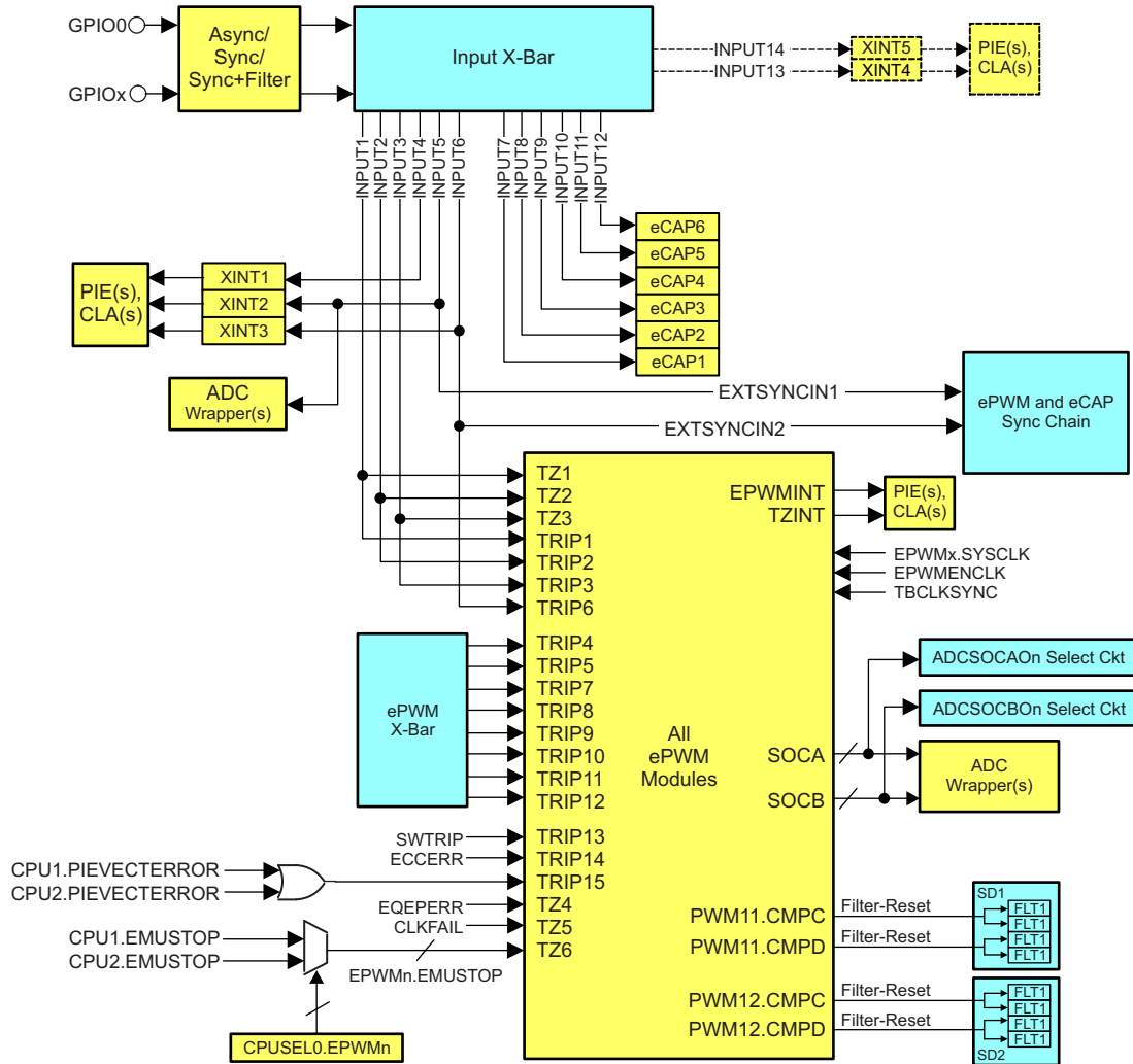
Figure 6-14. ePWM
