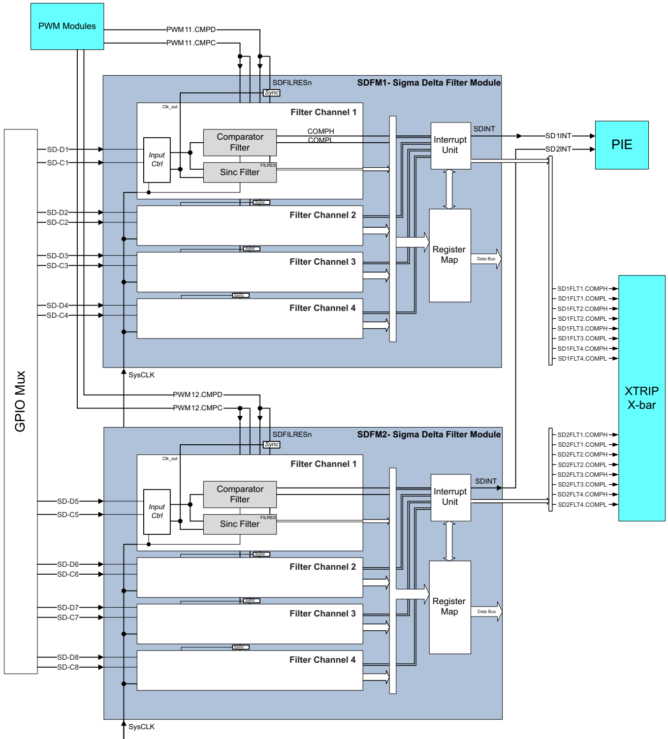
Figure 6-12. SDFM
