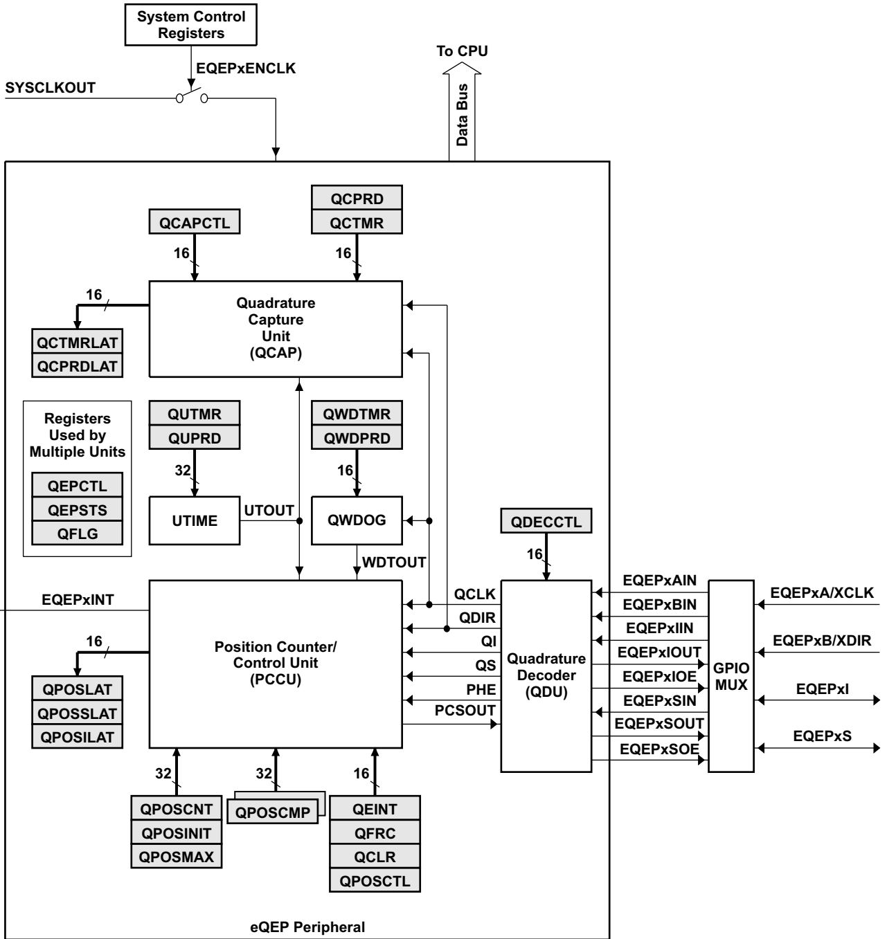
Figure 6-17. eQEP Block Diagram
