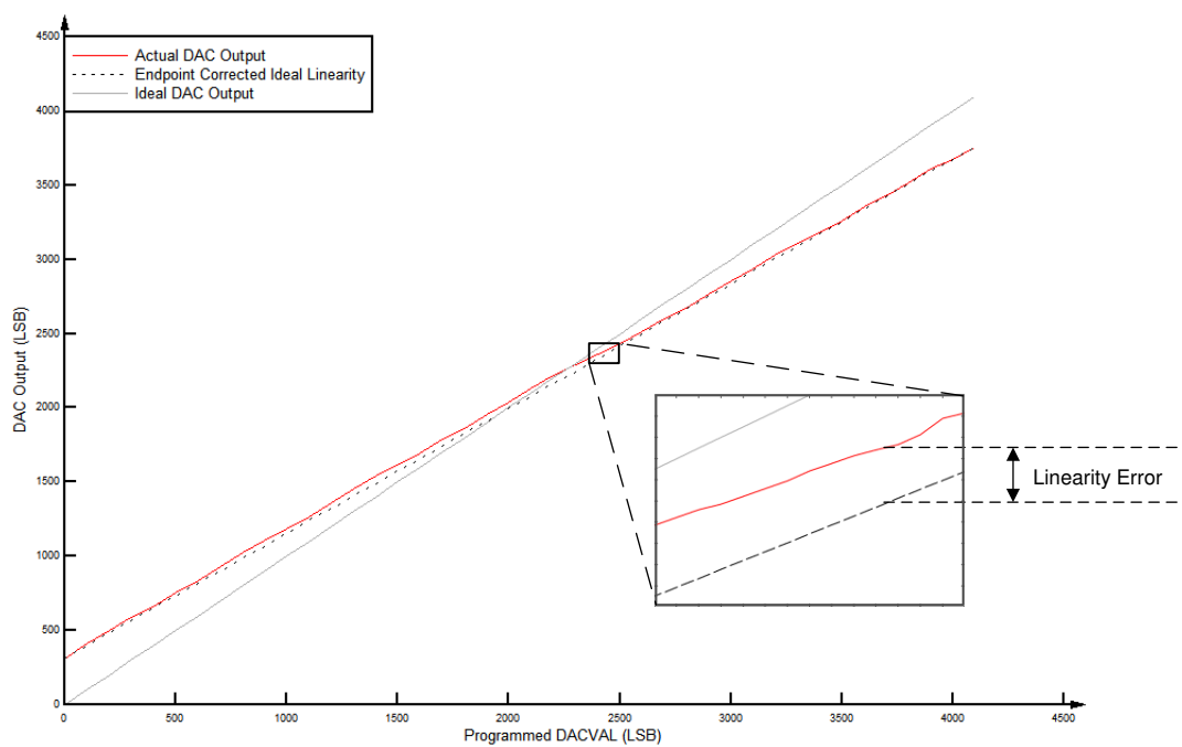
Figure 8-43. CMPSS DAC Static Linearity
