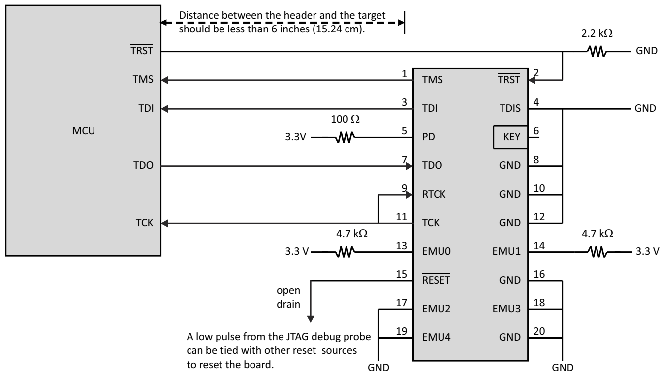
Figure 8-10. Connecting to the 20-Pin JTAG Header
