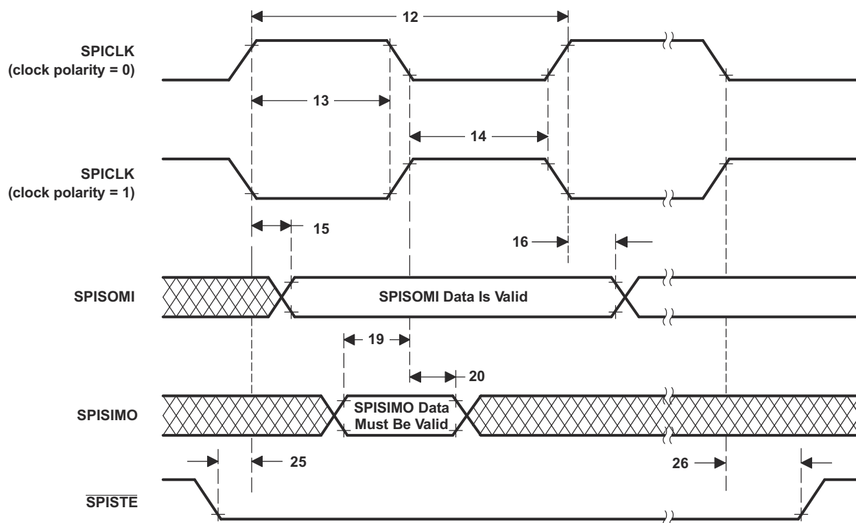
Figure 8-74. SPI Slave Mode External Timing (Clock Phase = 0)
