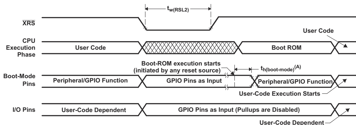
Figure 8-5. Power-on Reset
