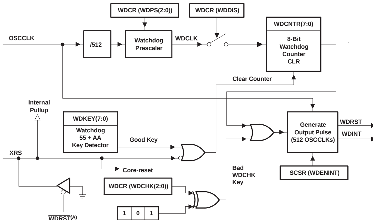
Figure 3-14. Watchdog Module
