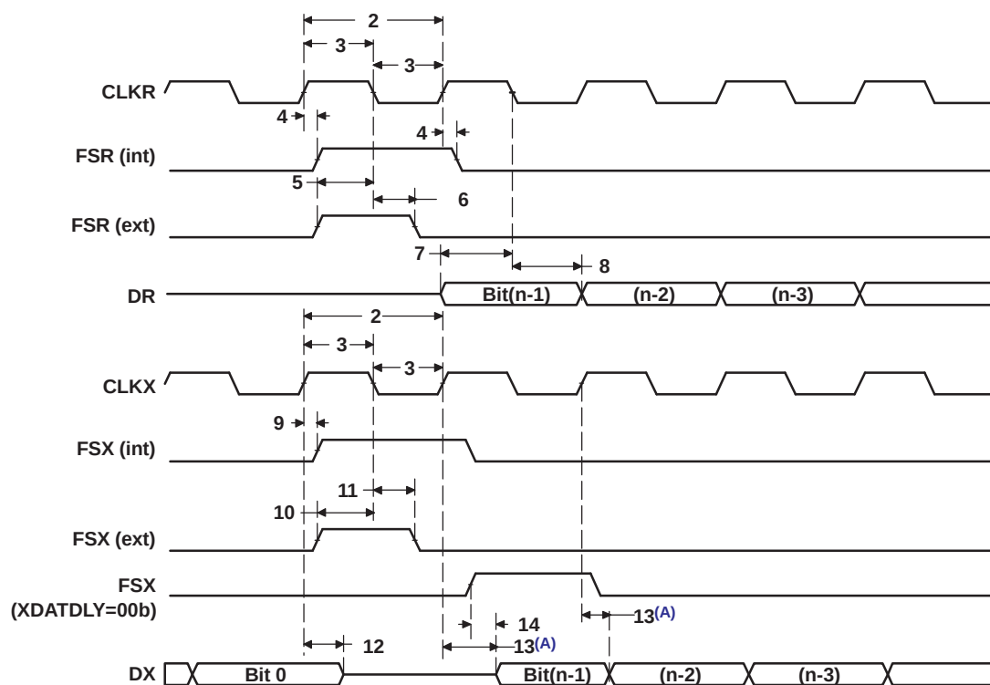
Figure 6-67. ASP Timing
