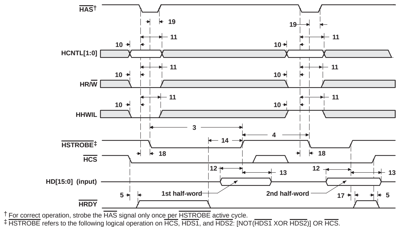
Figure 49. HPI Write Timing ( \overline{HAS} Used)
