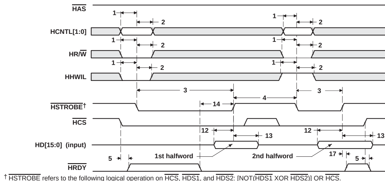
Figure 48. HPI Write Timing ( \overline{HAS} Not Used, Tied High)
