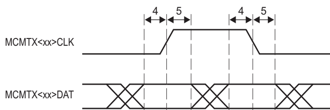
Figure 7-41 HyperLink Station Management Transmit Timing
