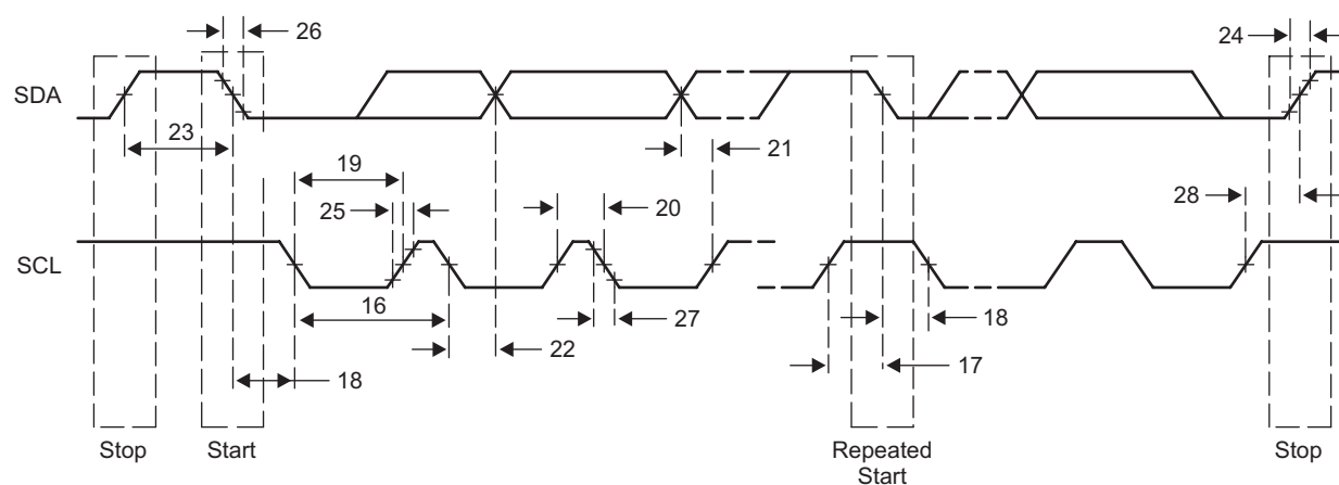
Figure 7-37 I 2 C Transmit Timings
