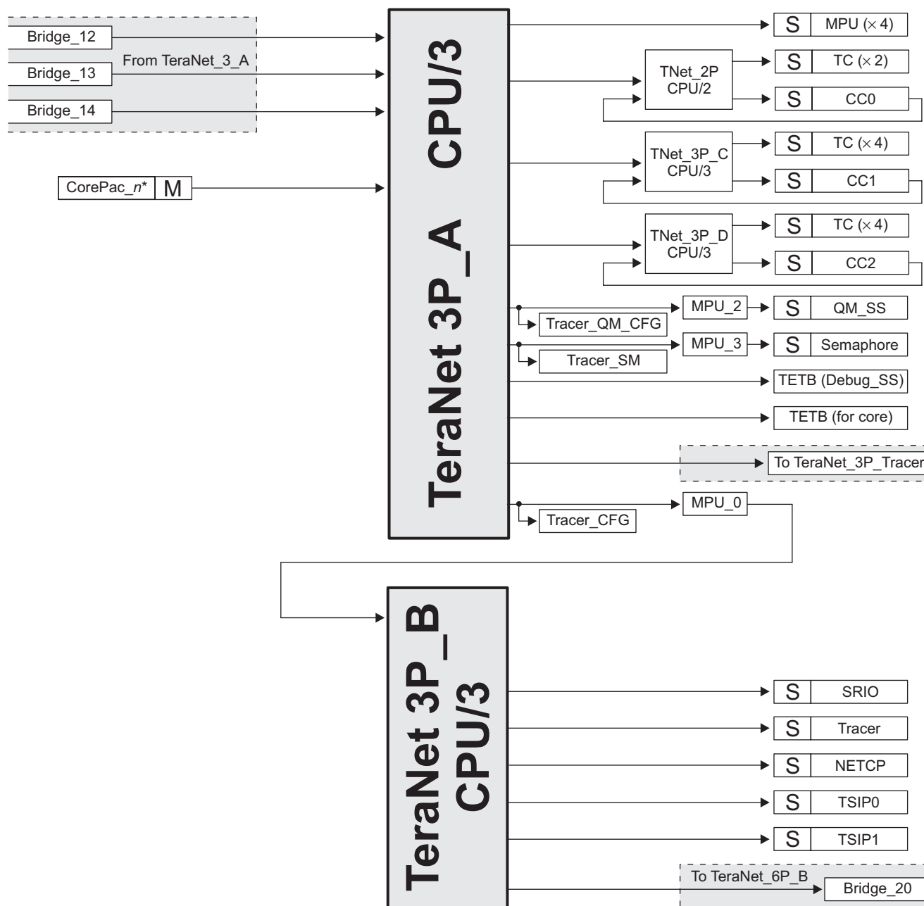
Figure 4-3 TeraNet 3P_A & B for C6678
