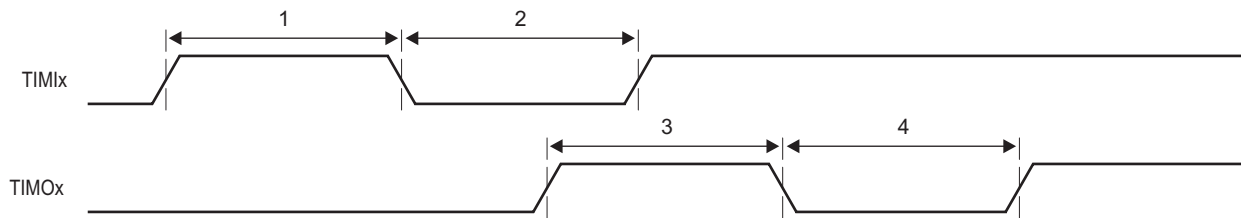
Figure 7-58 Timer Timing
