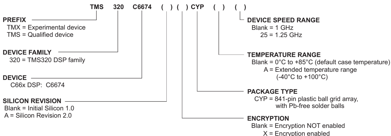
Figure 2-17 C66x DSP Device Nomenclature (including the TMS320C6674)
