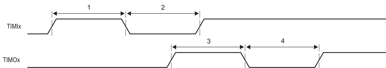
Figure 7-59 Timer Timing
