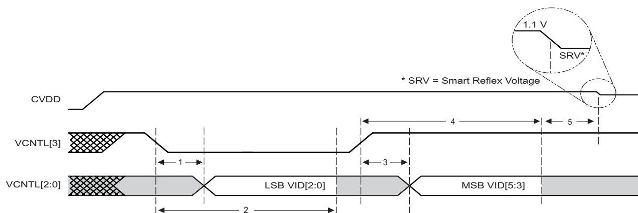
Figure 7-3 SmartReflex 4-Pin VID Interface Timing
