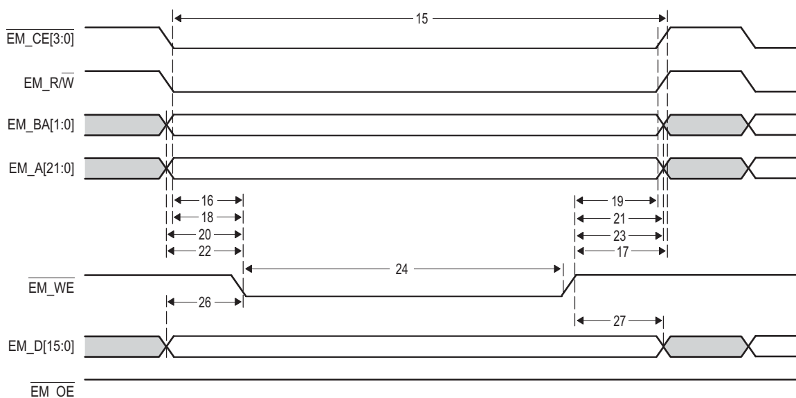
Figure 7-51 EMIF16 Asynchronous Memory Write Timing Diagram
