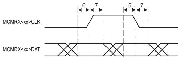
Figure 7-42 HyperLink Station Management Receive Timing
