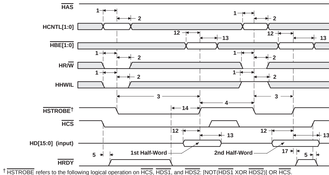
Figure 32. HPI Write Timing ( \overline{\text{HAS}} Not Used, Tied High)
