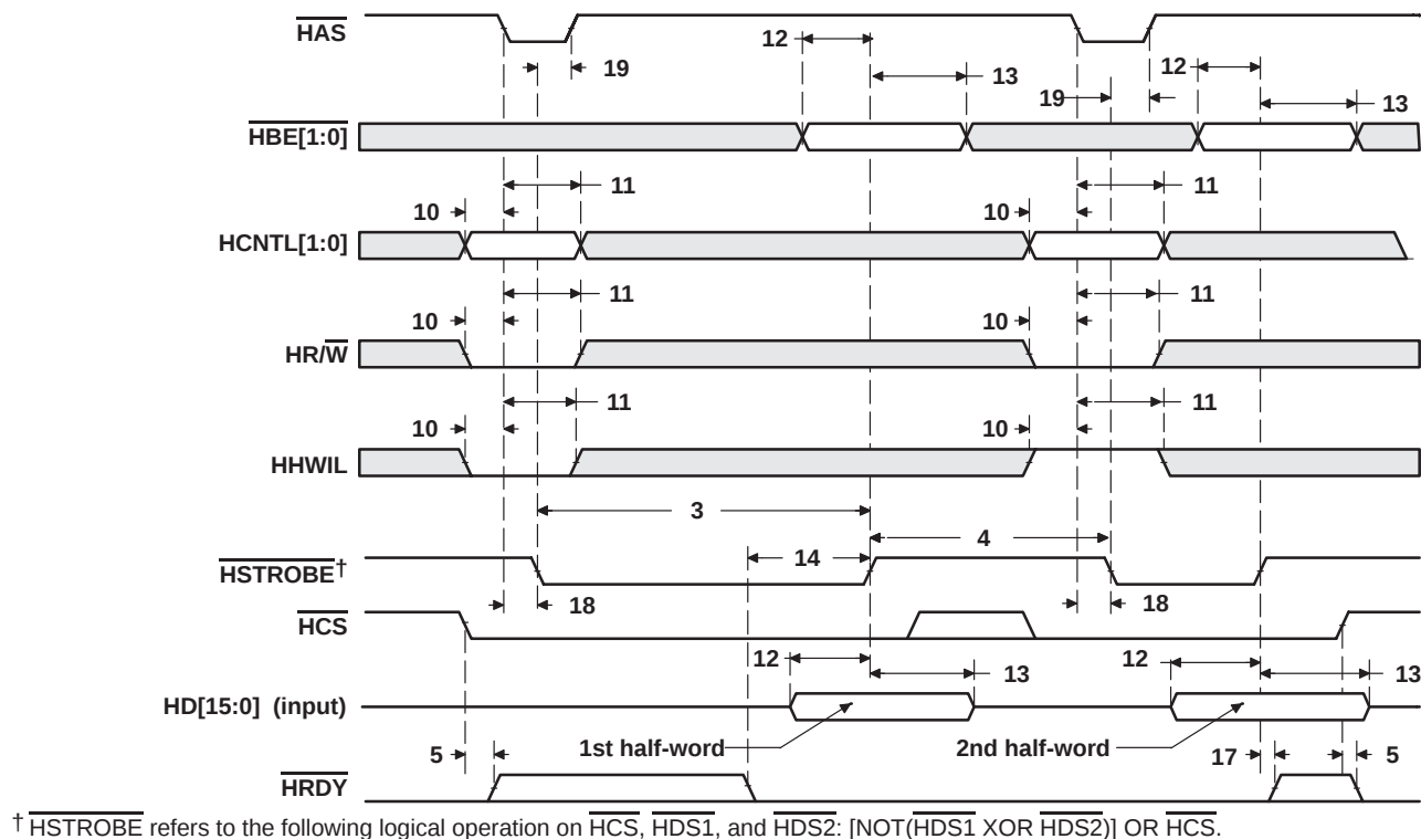
Figure 33. HPI Write Timing ( \overline{\text{HAS}} Used)
