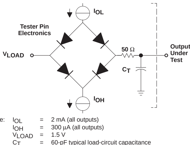
Figure 4. Test Load Circuit
