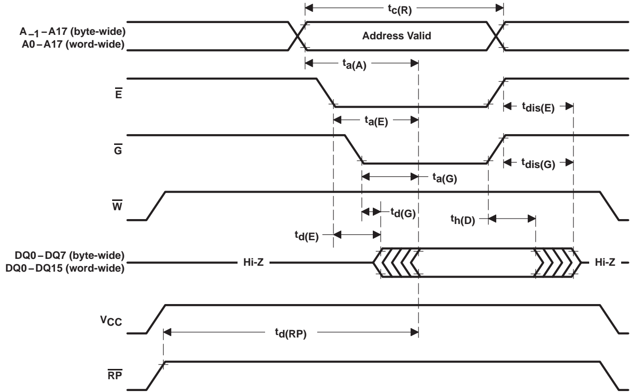
Figure 11. Read-Cycle Timing
