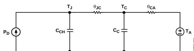
Figure 23. Thermal Circuit Model
