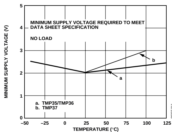
Figure 10. Minimum Supply Voltage vs. Temperature
