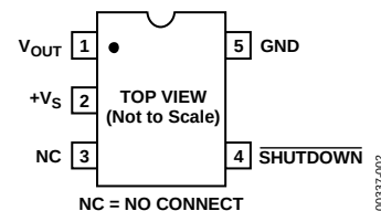
Figure 2. RT-5 (SOT-23)
