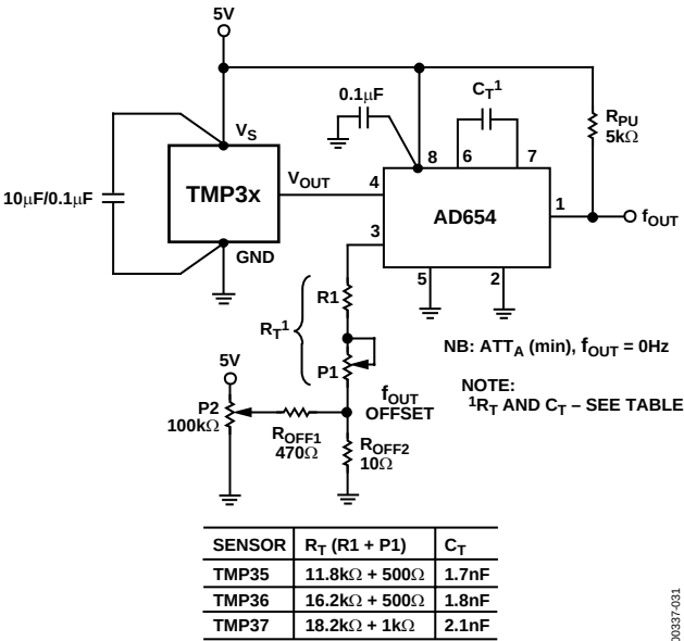
Figure 34. Temperature-to-Frequency Converter
