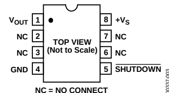
Figure 3. RN-8 (SOIC)
