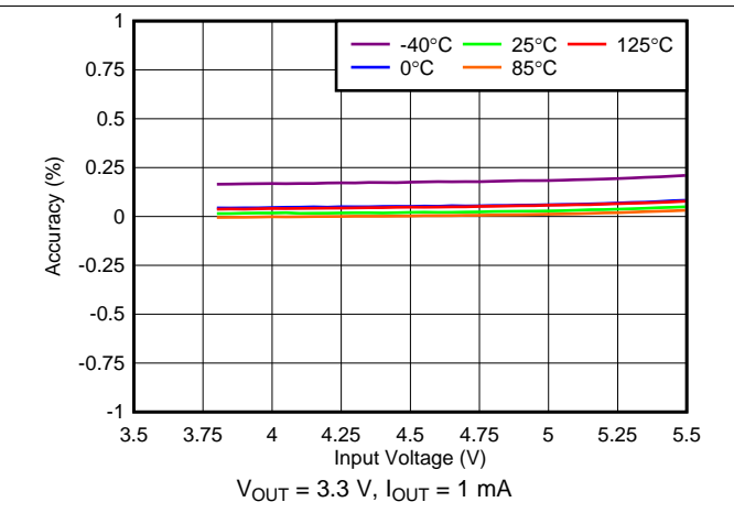
图 16. 3.3 V Regulation vs V_{IN} (Line Regulation)
