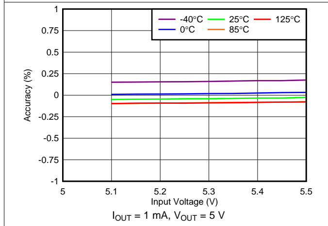
图 17. 5.0-V Accuracy vs V_{IN} (Line Regulation)
