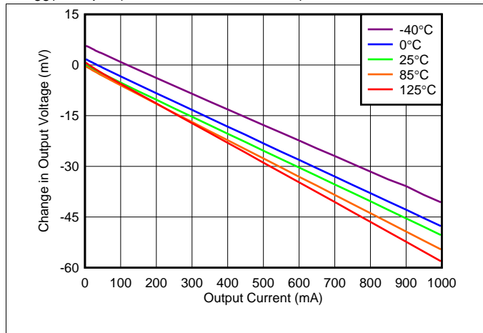
图 13. Load Regulation vs I_{OUT}
