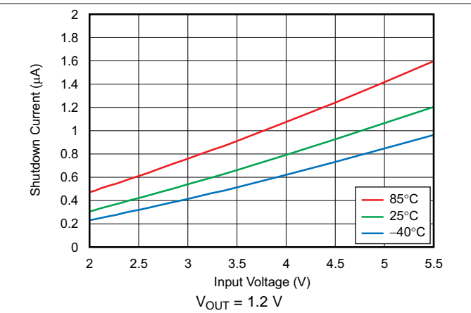
Figure 26. Shutdown Current vs Input Voltage
