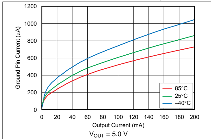
Figure 25. Ground Pin Current vs Output Current
