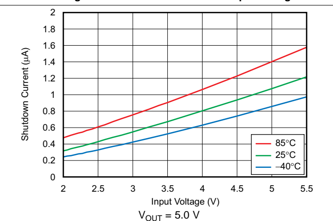
Figure 28. Shutdown Current vs Input Voltage
