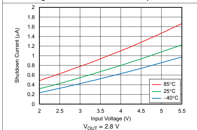
Figure 27. Shutdown Current vs Input Voltage
