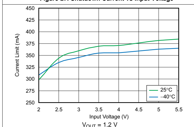
Figure 29. Current Limit vs Input Voltage
