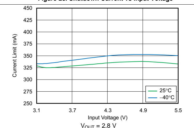
Figure 30. Current Limit vs Input Voltage
