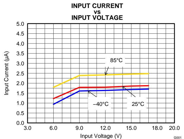
Figure 21. Shutdown Current
