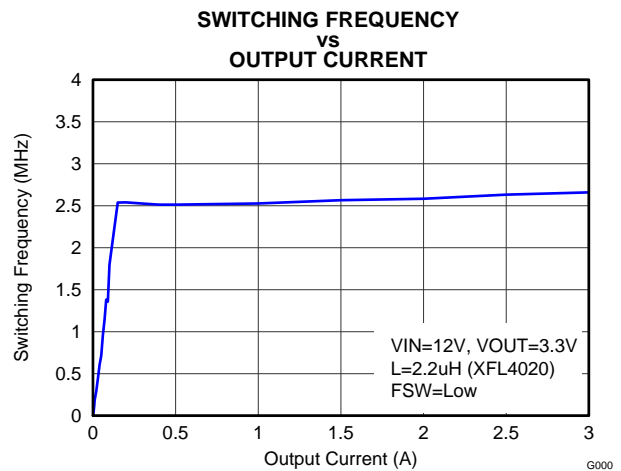
Figure 19. Switching Frequency
