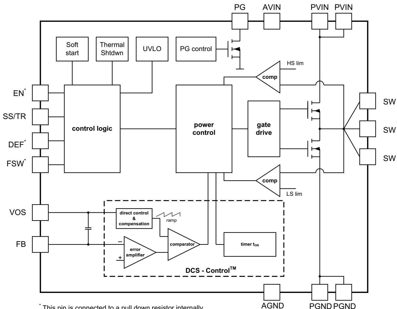
Figure 2. TLV62130
