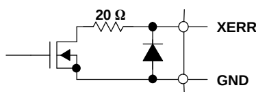
Figure 3. Output Equivalent Circuit (XERR)
