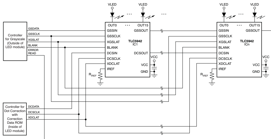
Typical Application Circuit (Multiple Daisy-Chaind TLC5942s)
