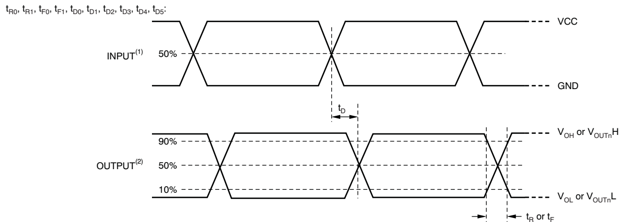
Figure 7. Input Timing
