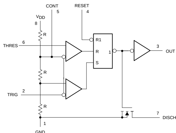
Simplified Schematic
