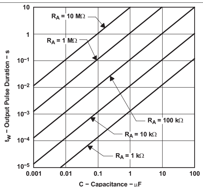
Figure 5. Output Pulse Duration vs Capacitance
