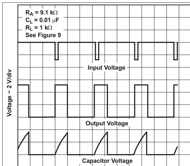
Figure 4. Typical Monostable Waveforms
