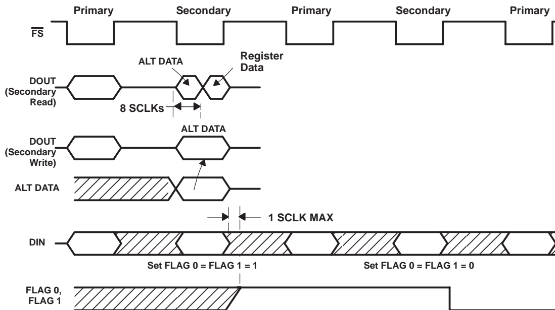
Figure 3–8. Phone Mode Timing
