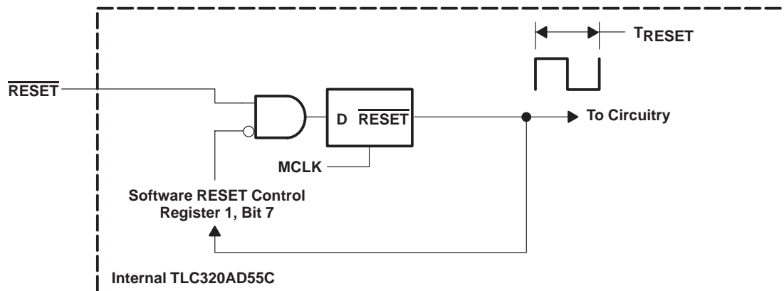
Figure 2–1. Reset Function
