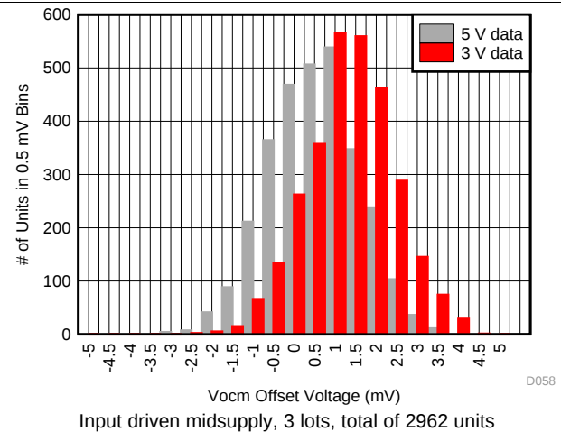
Figure 58. Common-Mode Output Offset from Driven V_{ocm}
