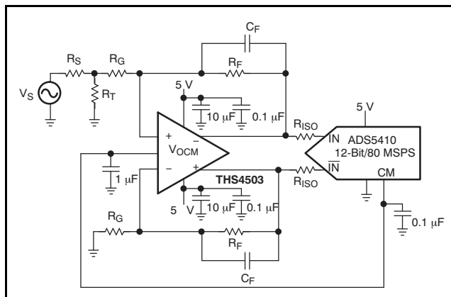
Figure 101. Using the THS4503 With the ADS5410
