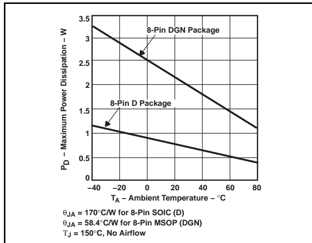
Figure 113. Maximum Power Dissipation vs Ambient Temperature
