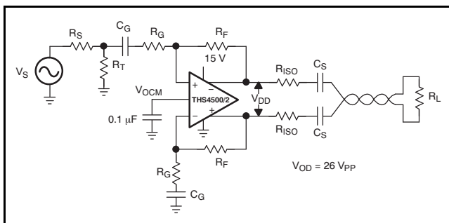
Figure 103. Fully Differential Line Driver With High Output Swing
