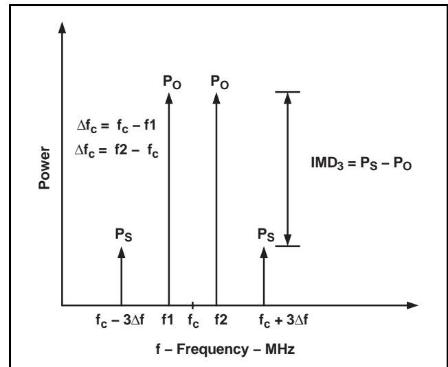
Figure 107. 2-Tone and 3rd-Order Intermodulation Products
