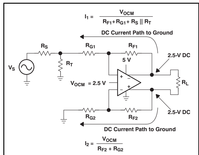
Figure 106. Depiction of DC Power Dissipation Caused By Output Level-Shifting in a DC-Coupled Circuit
