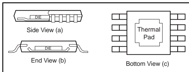
Figure 111. Views of PowerPAD, Thermally-Enhanced Package
