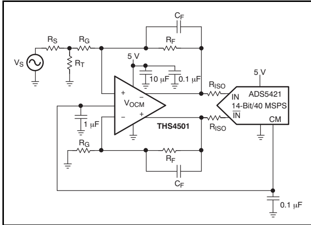
Figure 102. Using the THS4501 With the ADS5421
