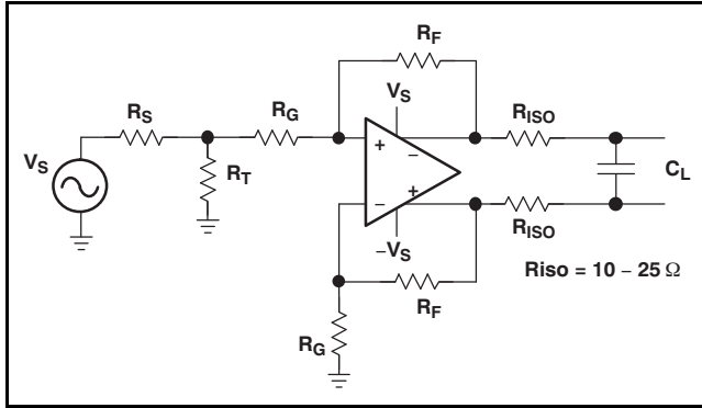
Figure 114. Use of Isolation Resistors With a Capacitive Load
