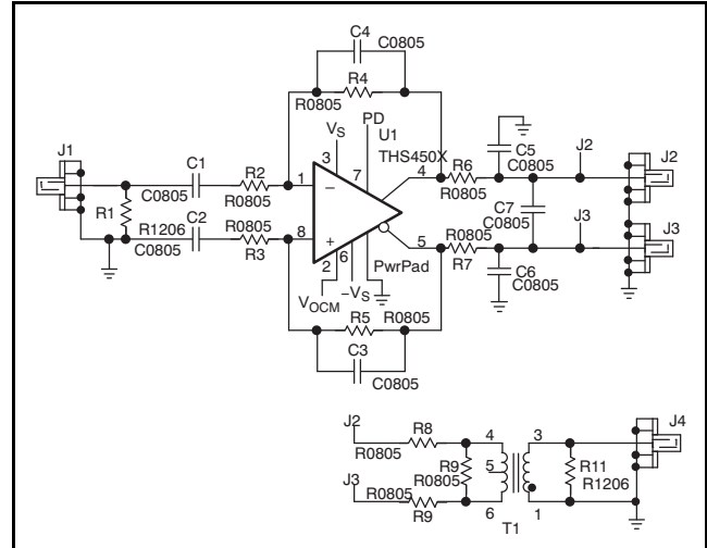
Figure 115. Simplified Schematic of the Evaluation Board
