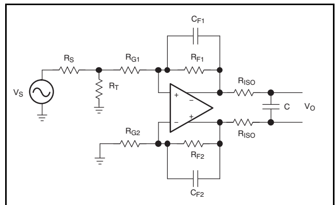
Figure 104. A Two-Pole, Low-Pass Filter Design Using a Fully Differential Amplifier With Poles Located at: P1 = (2\pi R_F C_F)^{-1} in Hz and P2 = (4\pi R_{ISO} C)^{-1} in Hz
