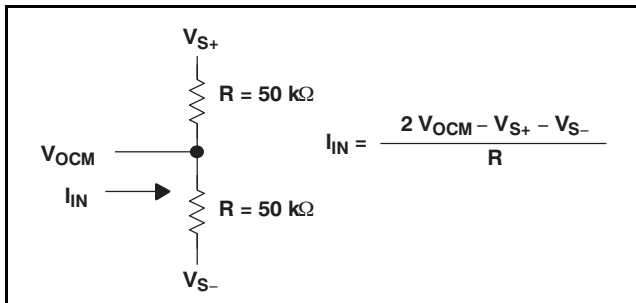
Figure 105. Equivalent Input Circuit for V_{OCM}
