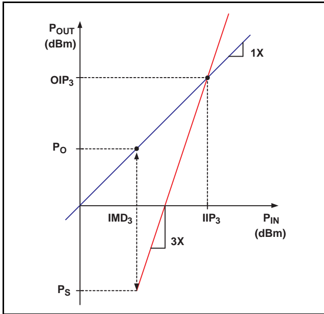
Figure 108. Graphical Representation of 2-Tone and 3rd-Order Intercept Point
