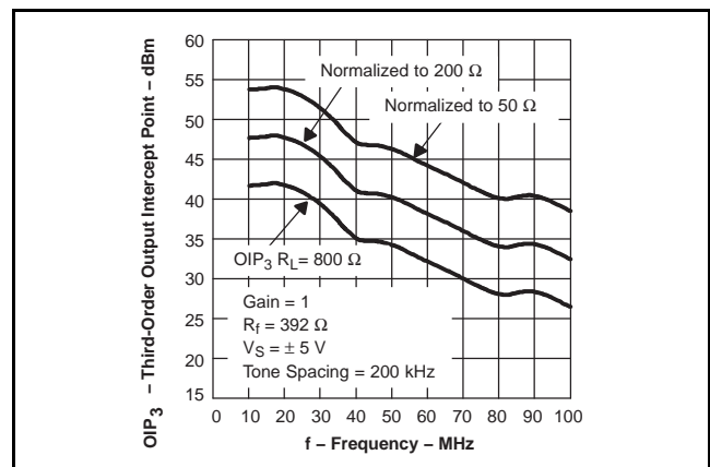
Figure 109. Equivalent 3rd-Order Intercept Point for the THS4500
