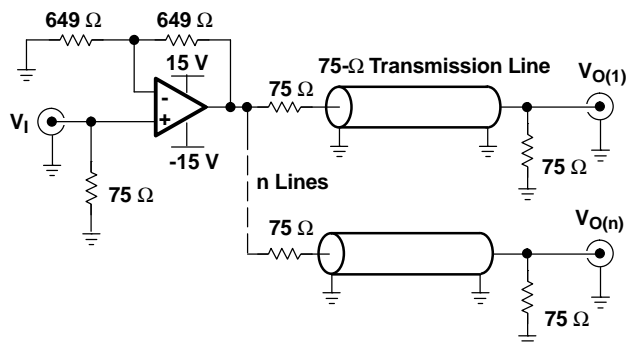
Figure 50. Video Distribution Amplifier Application
