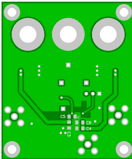
Figure 64. THS3120 EVM Board Layout (Bottom Layer)
