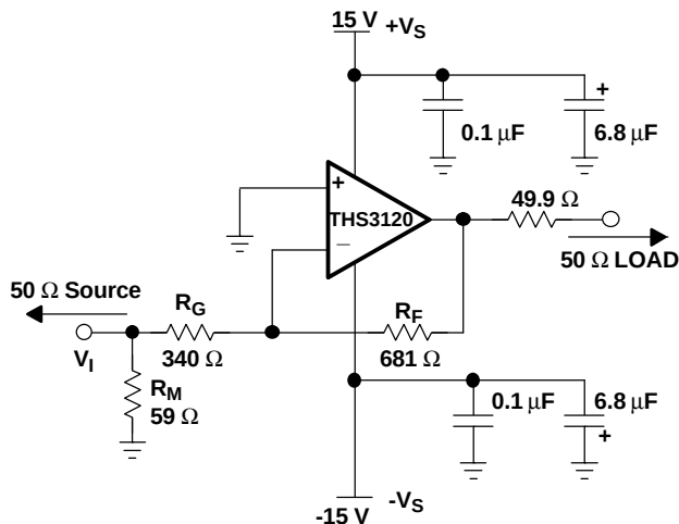
Figure 48. Wideband, Inverting Gain Configuration
