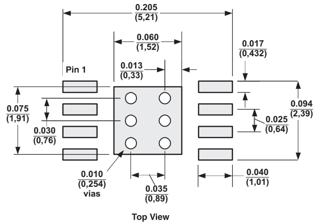
Figure 56. DGN PowerPAD PCB Etch and Via Pattern Dimensions are in inches (mm)
