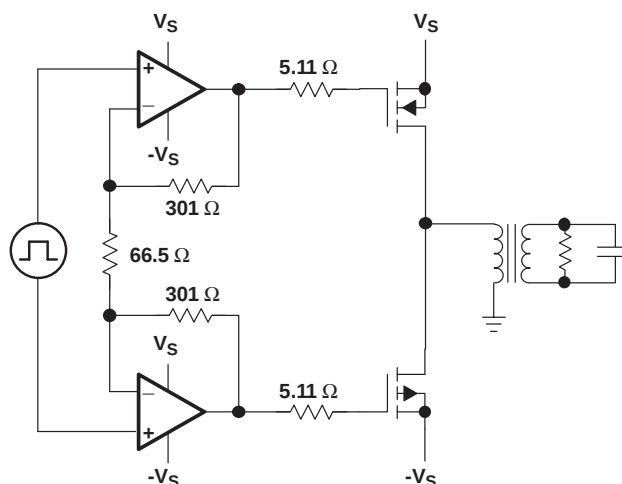
Figure 53. PowerFET Drive Circuit
