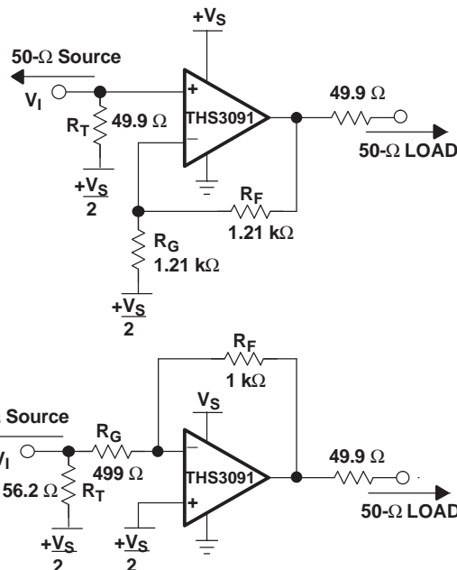
Figure 61. DC-Coupled, Single-Supply Operation
