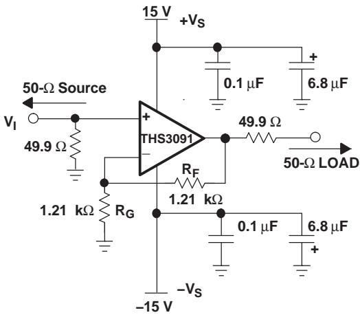
Figure 59. Wideband, Noninverting Gain Configuration
