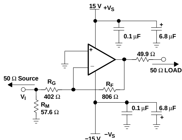
Figure 53. Wideband, Inverting Gain Configuration
