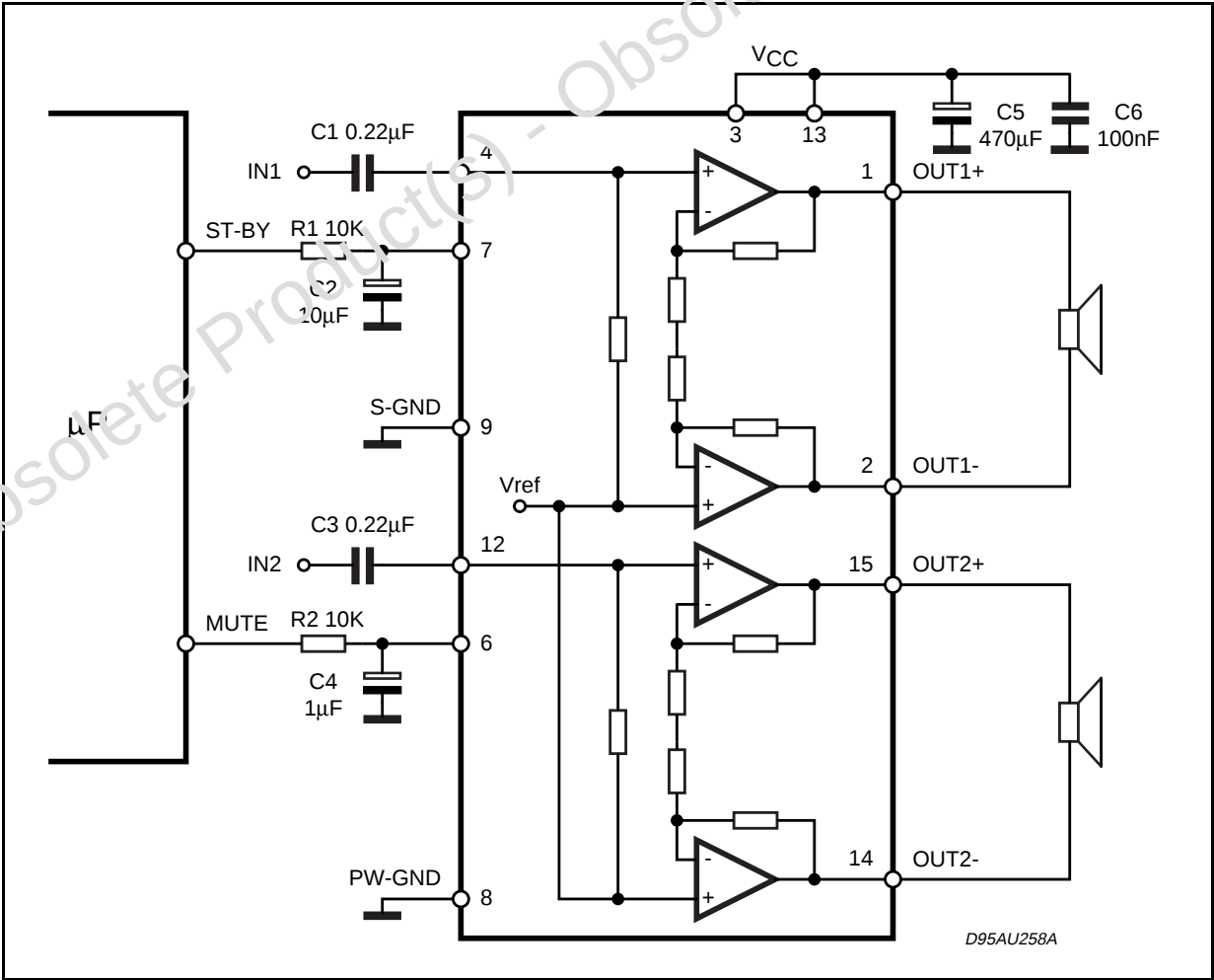
Figure 1: Microprocessor Application
