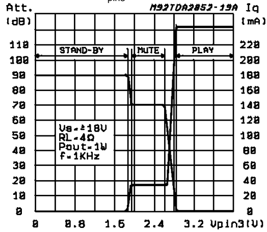
Figure 10: Output Attenuation & Quiescent Current vs. V_{pin3} .
