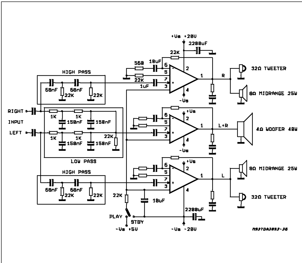
Figure 18: Multiway Application Circuit
