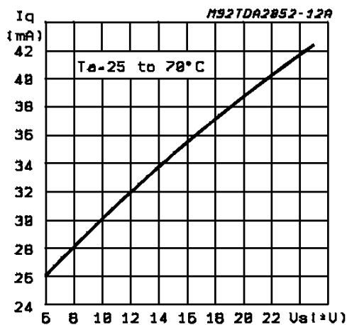
Figure 7: Quiescent Current vs. Supply Voltage
