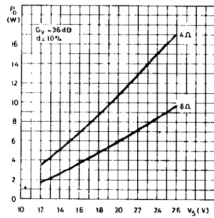
Figure 4 : Output Power versus Supply Voltage
