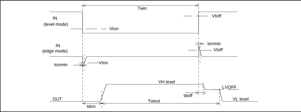
Figure 5: Minimum ON-time
