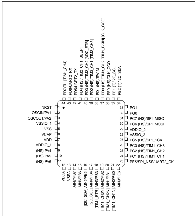
Figure 4: LQFP 44-pin pinout
