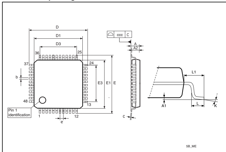
Figure 50. LQFP48 – 7 x 7 mm, 48-pin low-profile quad flat package outline (1)
