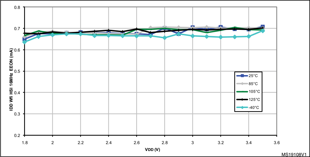
Figure 16. Typical I_{DD(Wait)} from Flash (HSI clock source), f_{CPU} = 16\text{ MHz}
