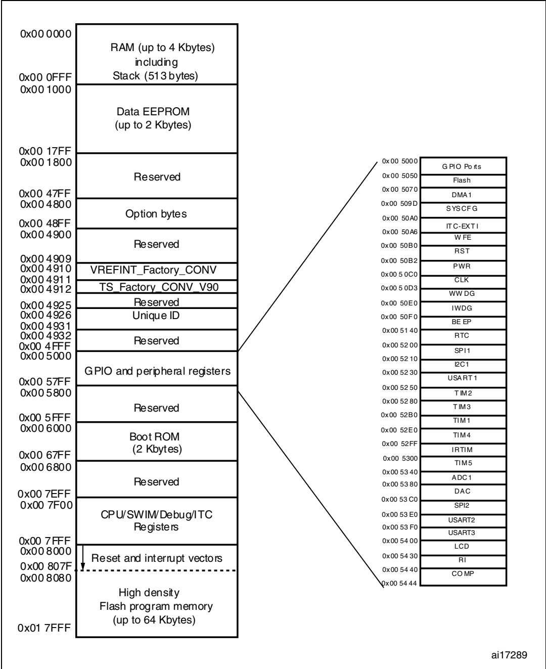
Figure 9. Memory map
