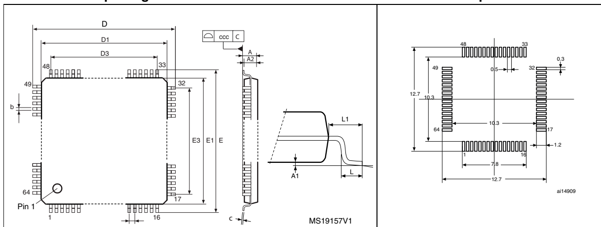
Figure 48. LQFP64 – 10 x 10 mm, 64 pin low-profile quad flat package outline (1)
