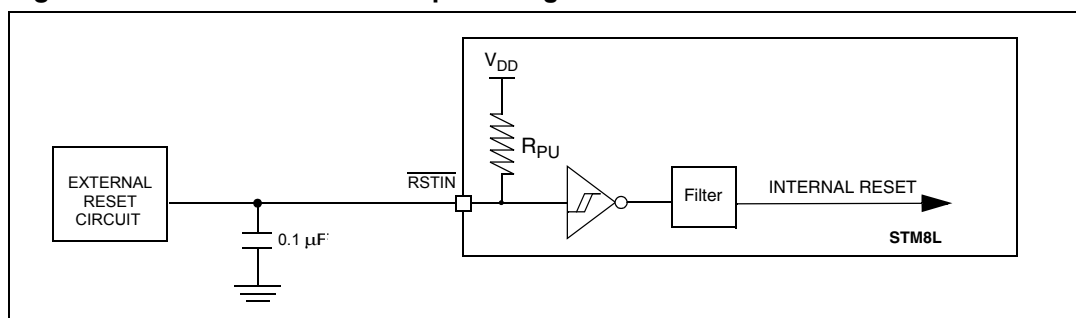
Figure 37. Recommended NRST pin configuration
