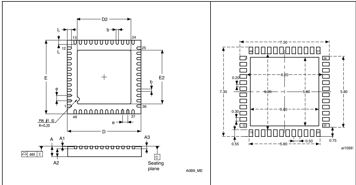
Figure 52. UFQFPN48 7 x 7 mm, 0.5 mm pitch, package outline (1)(2)(3) Figure 53. Recommended footprint (dimensions in mm) (1)
