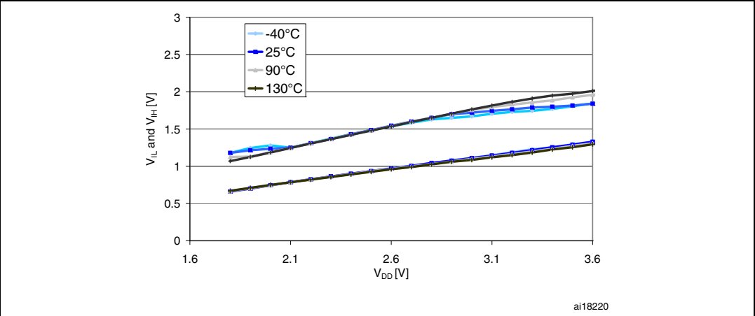
Figure 25. Typical V_{IL} and V_{IH} vs. V_{DD} (standard I/Os)
