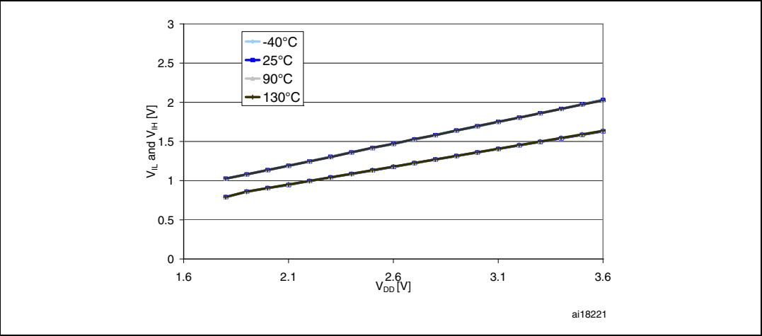
Figure 26. Typical V_{IL} and V_{IH} vs. V_{DD} (true open drain I/Os)
