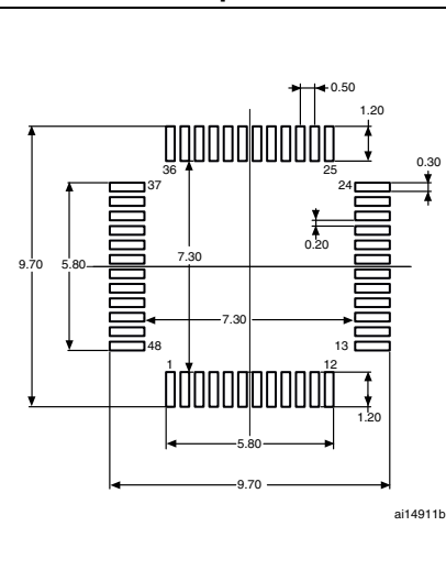
Figure 51. Recommended footprint (1)(2)
