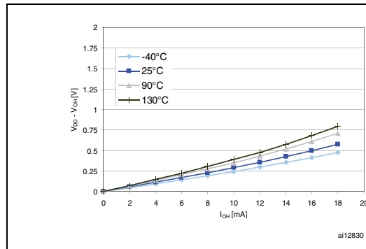
Figure 33. Typical V_{DD} - V_{OH} @ V_{DD} = 3.0\text{ V} (high sink ports)
