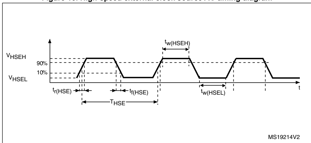
Figure 13. High-speed external clock source AC timing diagram
