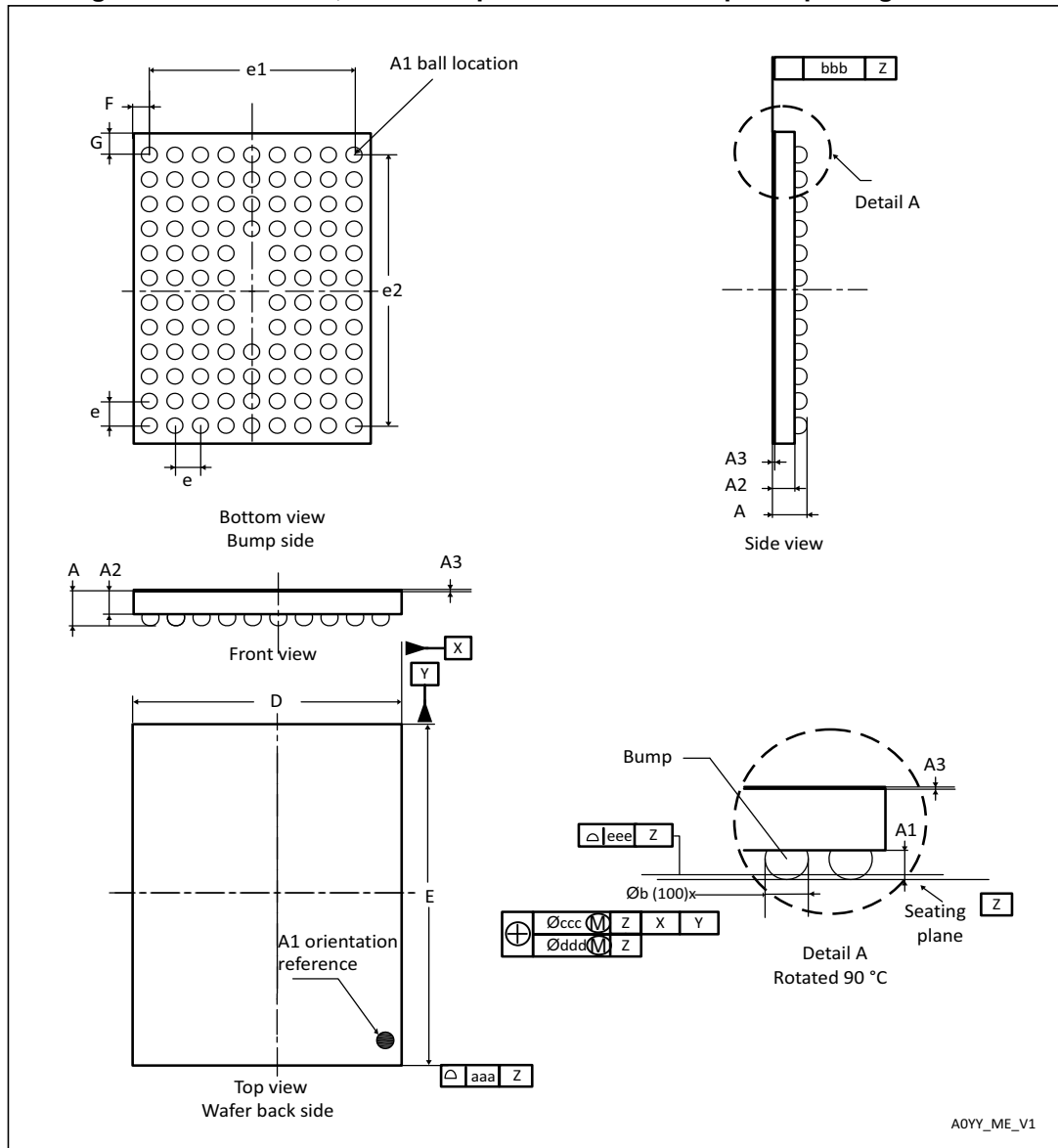
Figure 39. WLCSP104, 0.400 mm pitch wafer level chip size package outline
