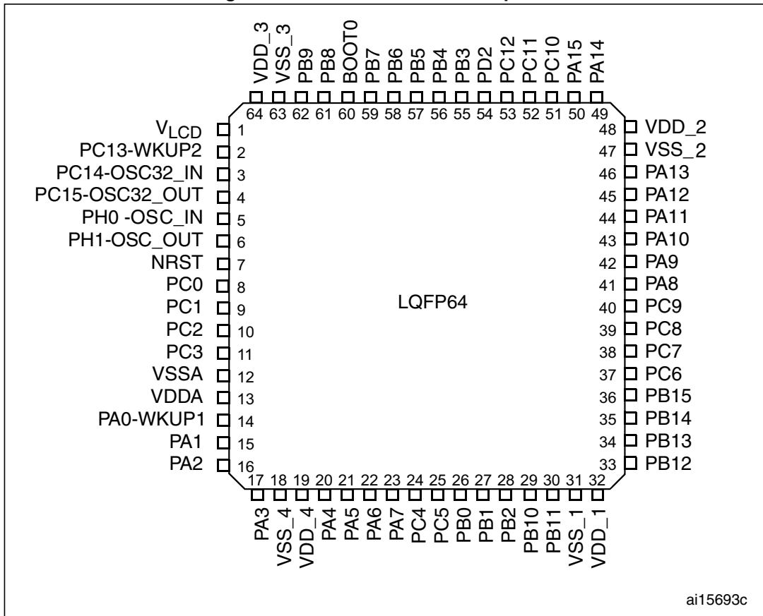
Figure 5. STM32L162RE LQFP64 pinout
