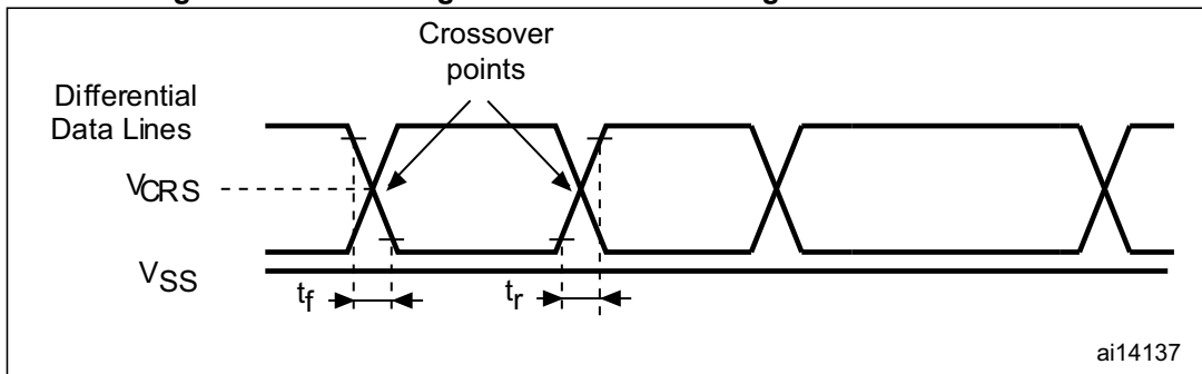
Figure 23. USB timings: definition of data signal rise and fall time
