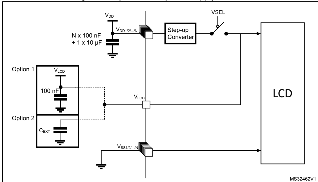
Figure 11. Optional LCD power supply scheme
