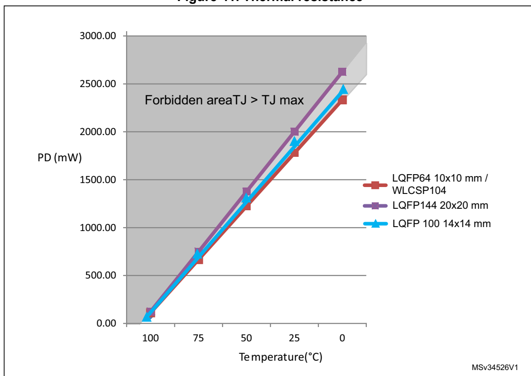
Figure 41. Thermal resistance
