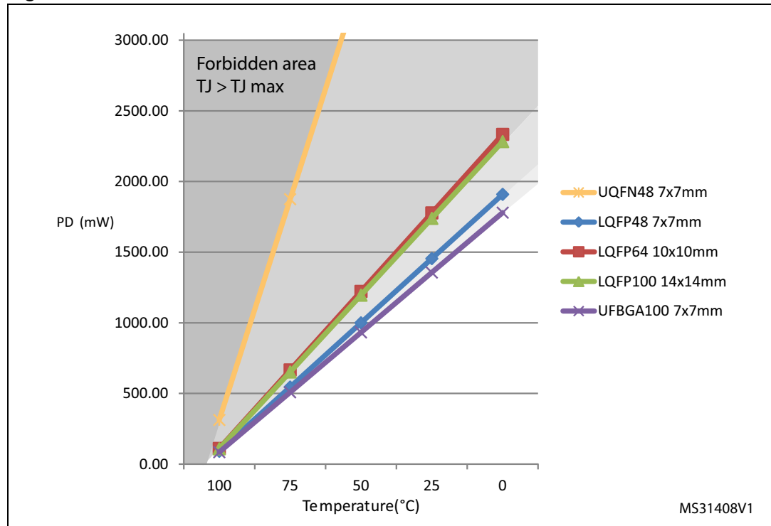
Figure 42. Thermal resistance
