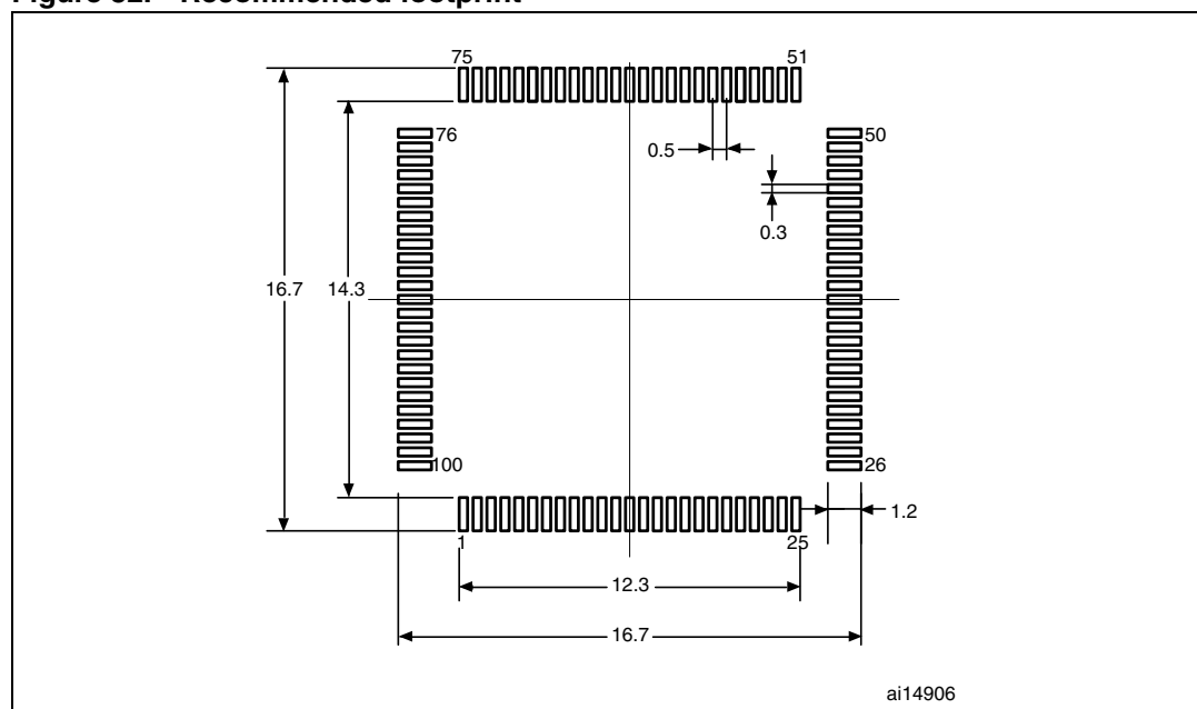
Figure 32. Recommended footprint
