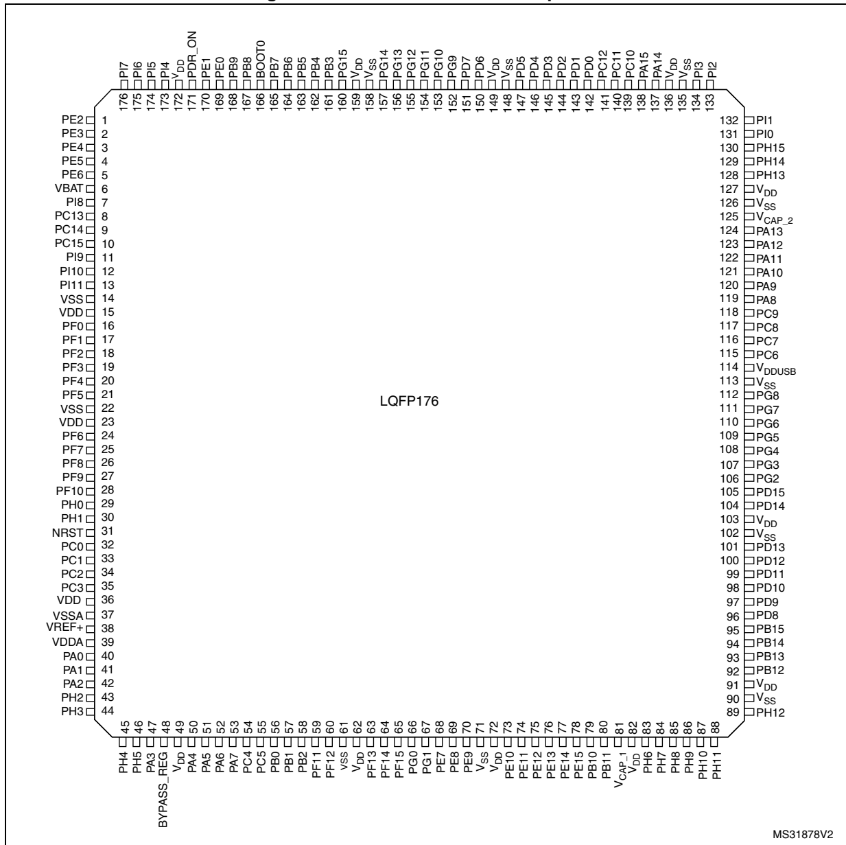
Figure 14. STM32F756lx LQFP176 pinout
