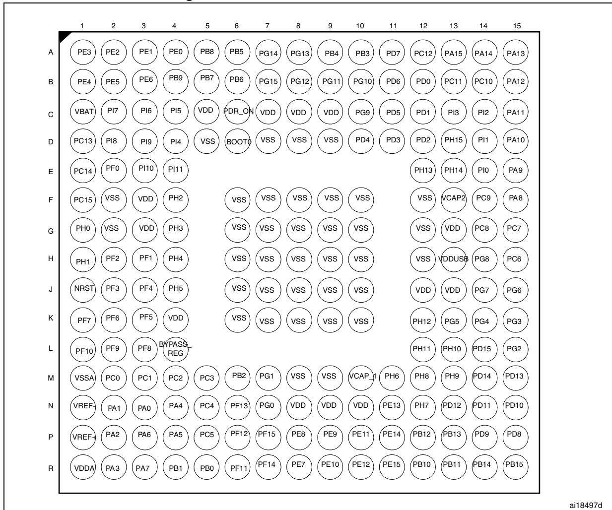
Figure 16. STM32F756lx UFBGA176 ballout
