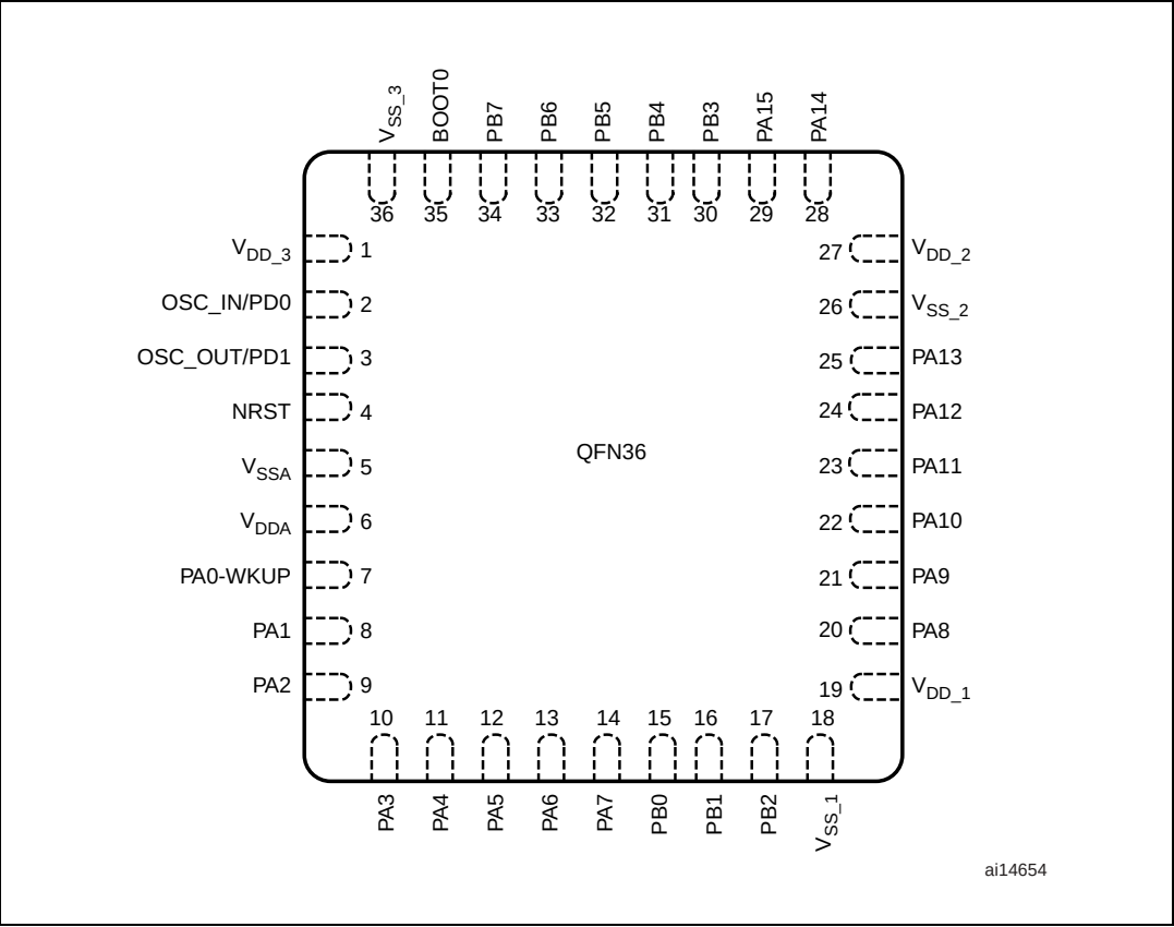
Figure 5. STM32F101xx access line VFQFPN36 pinout
