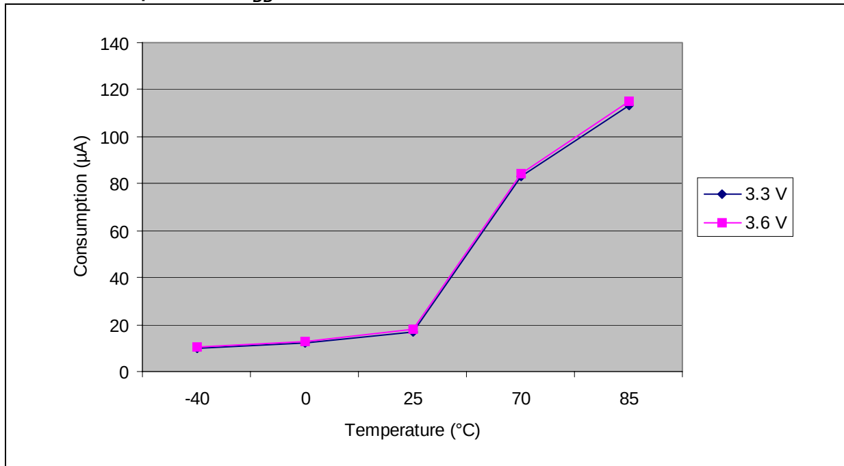
Figure 14. Current consumption in Stop mode with regulator in Low-power mode versus temperature at V_{DD} = 3.3\text{ V} and 3.6\text{ V}
