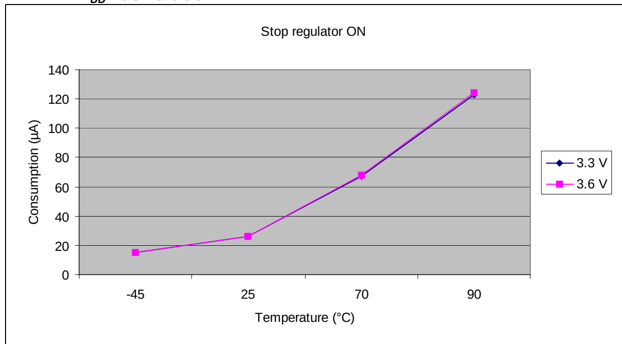
Figure 13. Current consumption in Stop mode with regulator in Run mode versus temperature at V_{DD} = 3.3\text{ V} and 3.6\text{ V}
