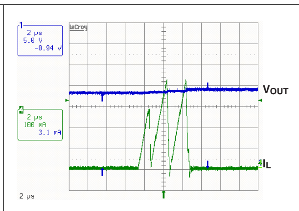
Figure 17. Overvoltage protection
