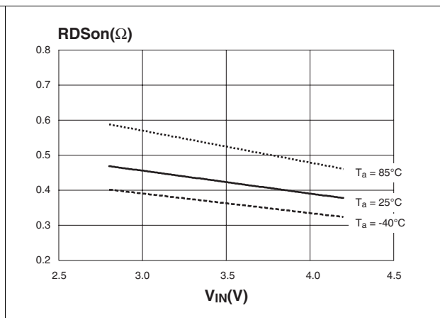
Figure 8. Boost switch resistance (STLD20D-DEF) vs VIN(V) for three temperatures: Ta = 85°C, 25°C, and -40°C.
