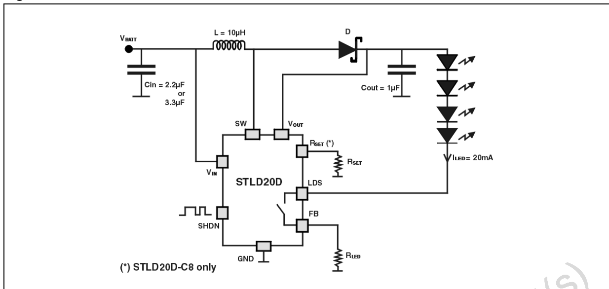
Figure 3. Basic connection
