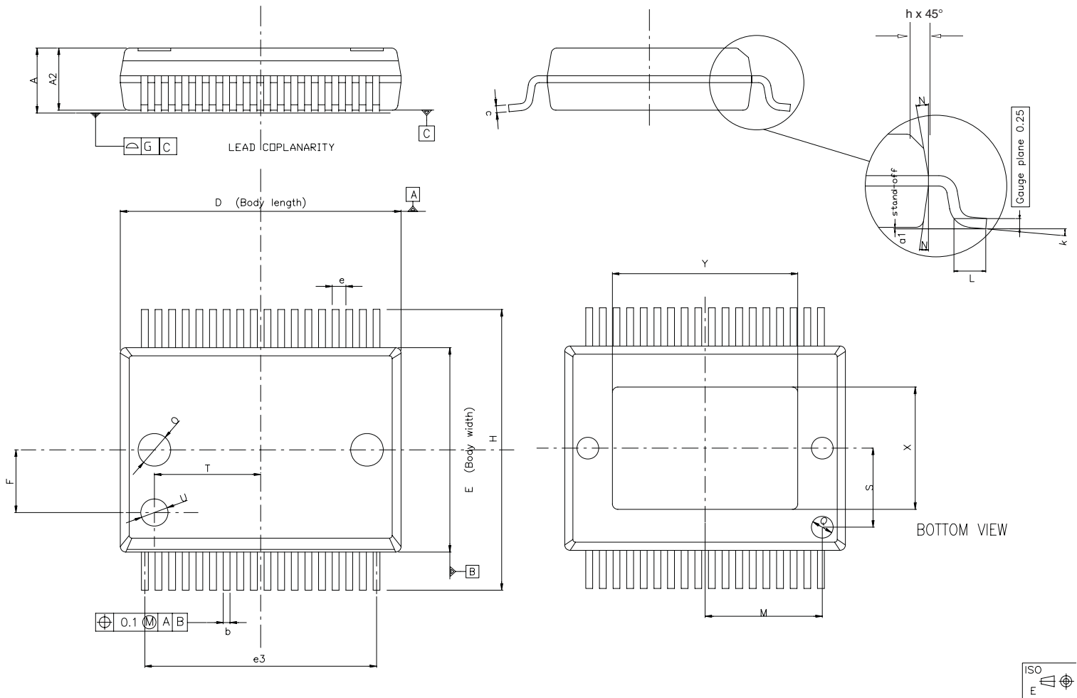
Figure 37. PowerSSO-36 EPD outline drawing
