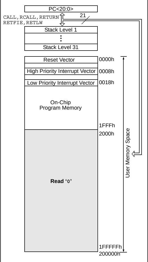
FIGURE 5-2: PROGRAM MEMORY MAP AND STACK FOR PIC18F1320
