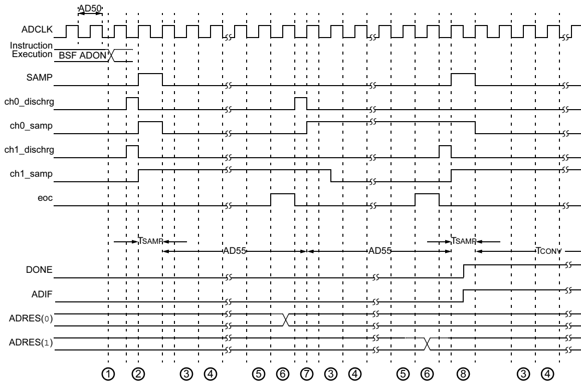
FIGURE 22-25: 10-BIT HIGH-SPEED A/D CONVERSION TIMING CHARACTERISTICS (CHPS = 01, SIMSAM = 0, ASAM = 1, SSRC = 111, SAMC = 00001)
