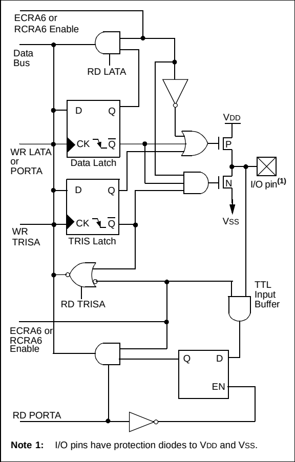
FIGURE 9-3: BLOCK DIAGRAM OF RA6
