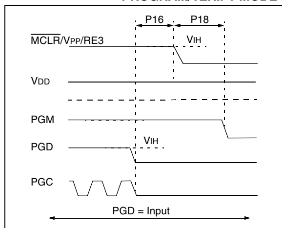
FIGURE 2-13: EXITING LOW-VOLTAGE PROGRAM/VERIFY MODE
