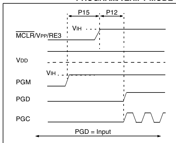
FIGURE 2-12: ENTERING LOW-VOLTAGE PROGRAM/VERIFY MODE
